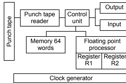
Figure 1 Z3 architecture of Zuse
